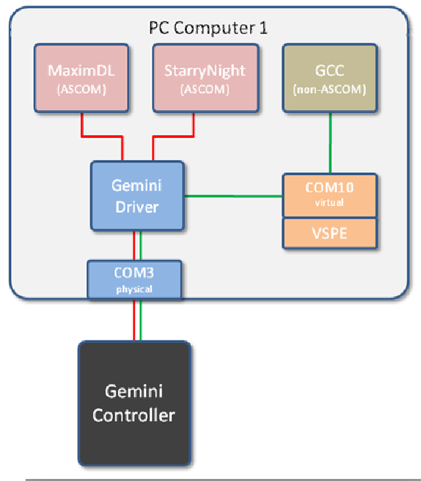
Pass-through configured to use a virtual COM port
